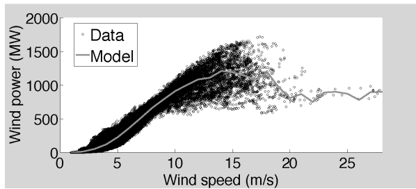
Figure 8. Power curves (left) and complementary cumulative probability distribution of wind output (right) for Imperial Valley for the deep integration study.
