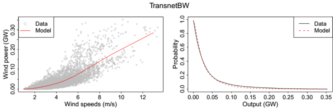
Figure 13. Power curves (left) and complementary cumulative probability distribution of wind output (right) for TransnetBW area.
