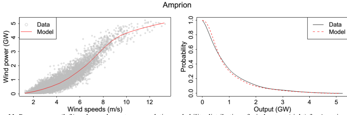
Figure 11. Power curves (left) and complementary cumulative probability distribution of wind output (right) for Amprion area.
