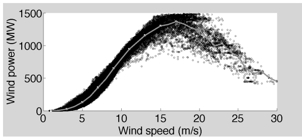
Figure 7. Power curves (left) and complementary cumulative probability distribution of wind output (right) for Clark County for the deep integration study.
