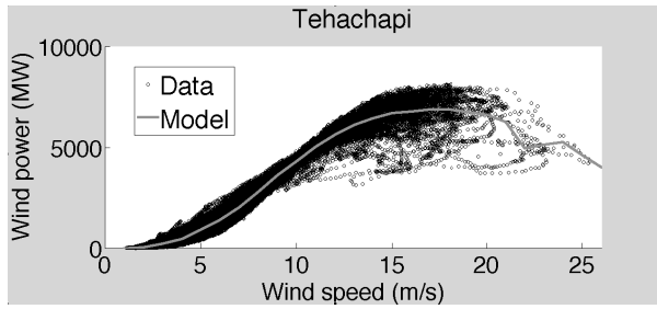
Figure 6. Power curves (left) and complementary cumulative probability distribution of wind output (right) for Tehachapi for the moderate (up) and deep (down) integration study.
