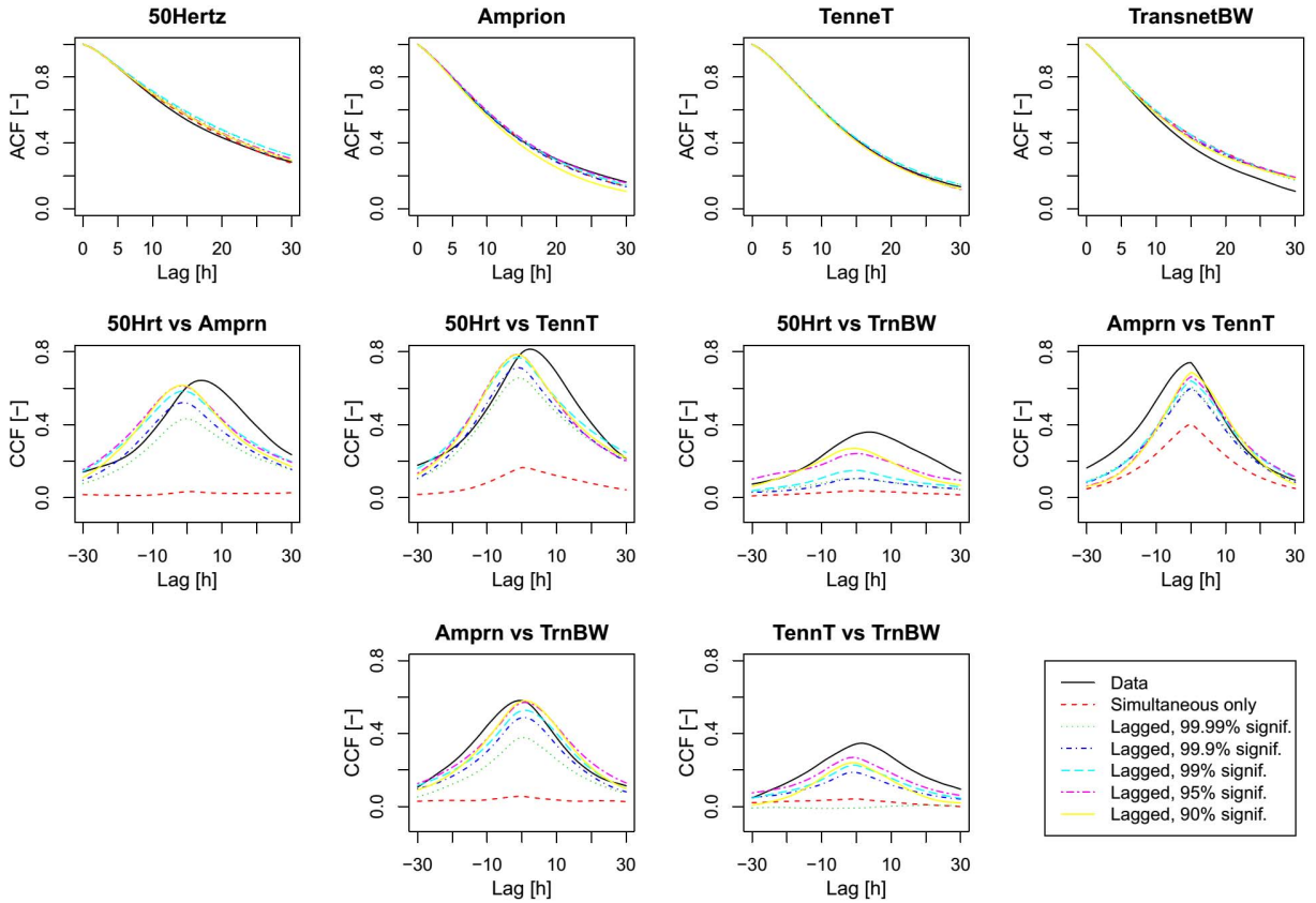
Figure 9. Auto-correlation (ACF) and cross-correlation functions (CCF) of the Gaussian noise y_{kt}^{GS} (transformed data) and simulated autoregressive noise Y_{kt}^{GS} , considering various significance threshold levels for the lagged cross-correlations. Germany case study.
