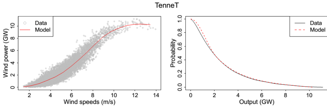
Figure 12. Power curves (left) and complementary cumulative probability distribution of wind output (right) for TenneT area.
