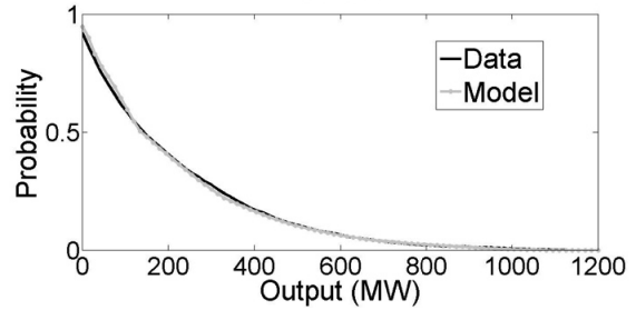
Figure 5. Power curves (left) and complementary cumulative probability distribution of wind output (right) for Solano for the moderate (up) and deep (down) integration study.
