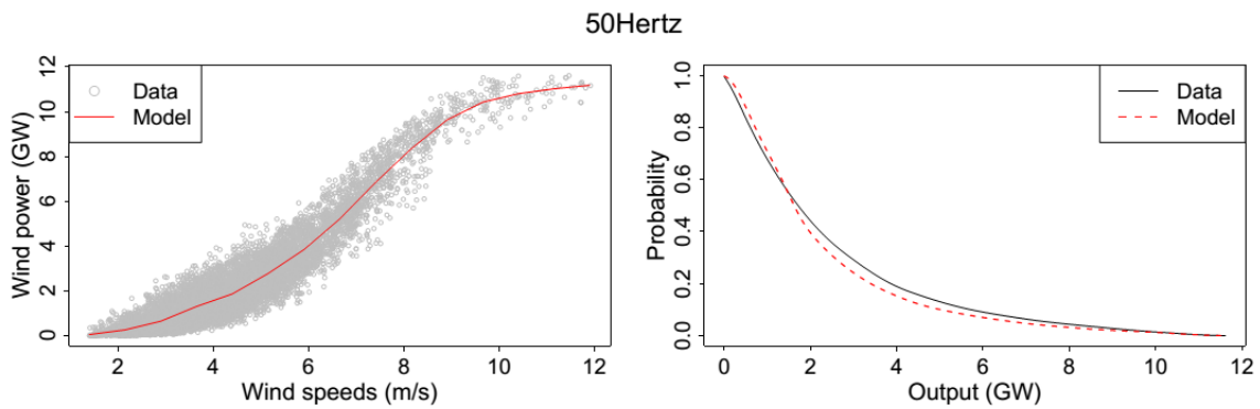
Figure 10. Power curves (left) and complementary cumulative probability distribution of wind output (right) for 50Hertz area.
