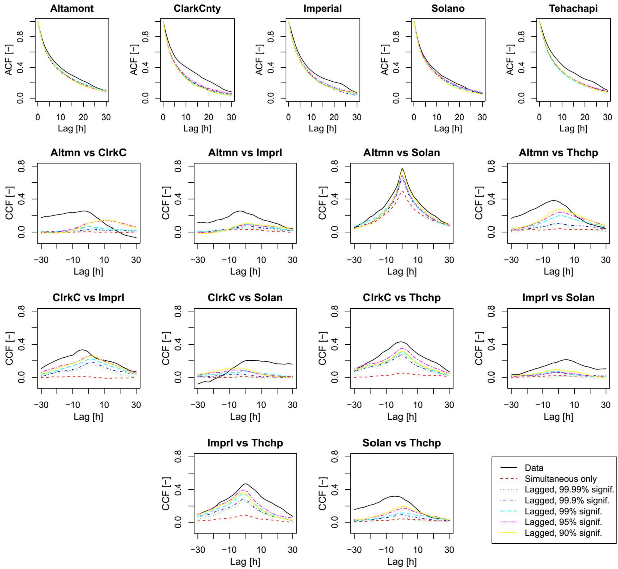
Figure 3. Auto-correlation (ACF) and cross-correlation functions (CCF) of the Gaussian noise y_{kt}^{GS} (transformed data) and simulated autoregressive noise Y_{kt}^{GS} , considering various significance threshold levels for the lagged cross-correlations. California deep integration case study.
