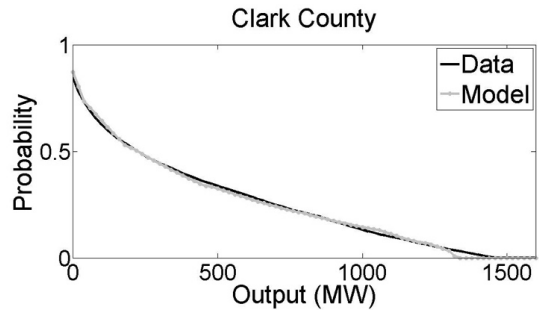
Figure 7. Power curves (left) and complementary cumulative probability distribution of wind output (right) for Clark County for the deep integration study.
